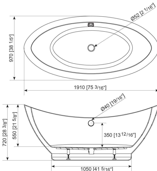
KOAN 1910 [75 3/16"] x 970 [38 1/5"]
