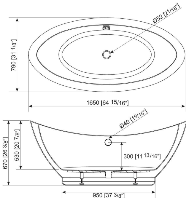
KOAN 1650 [64 15/16"] x 790 [31 1/8"]
